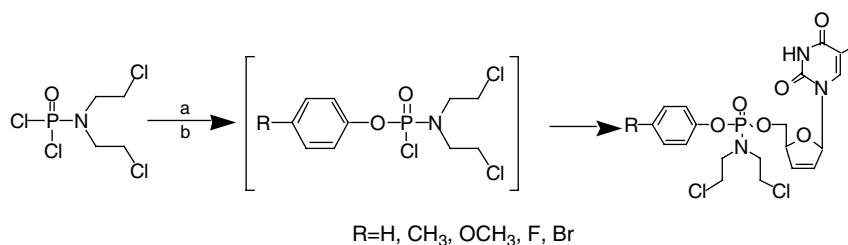
Scheme 1. Synthetic scheme for chloroethyl substituted phosphoramidate derivatives of stavudine. (a) Phenol, triethylamine, 1,2,4-triazole; (b) stavudine.
