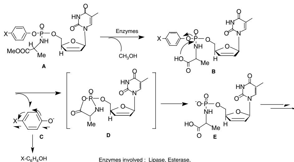
Figure 5. New Pathway for the lipase-mediated hydrolysis of phosphoramidate derivatives of stavudine based on various enzymes involved.
