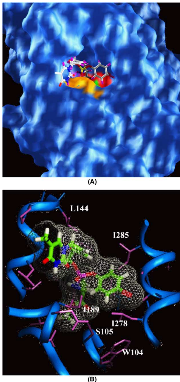
Figure 3. (A) The model of the S -stereoisomer of the stampidine molecule in the active site of the C. Antarctica lipase, a solid surface representation based on the crystal structure of the protein and the computation of energetically favored conformations for the ligand by a previously published docking procedure. 48–52 (B) The model of the S -stereoisomer of the stampidine molecule in the active site of the C. Antarctica lipase, based on the crystal structure of the protein and the computation of energetically favored conformations for the ligand by a previously published docking procedure. 48–52 The close-up view of the phenoxy ring interacting with the surrounding protein residues (labeled). Prepared with InsightII. 52
