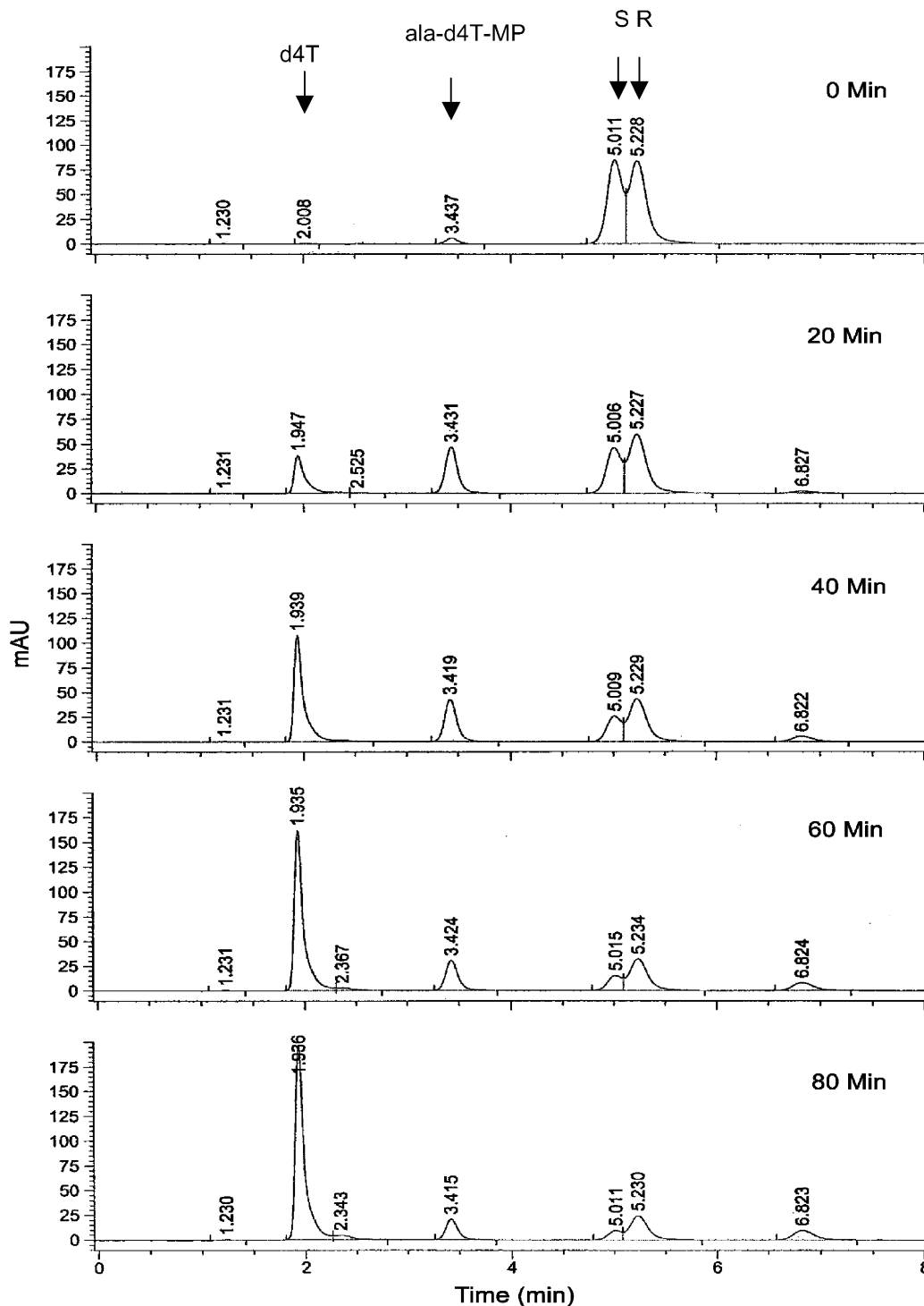
Figure 4. HPLC profiles of 4-fluoro phenylphosphoramidate derivative with lipase at various time intervals at room temperature.
