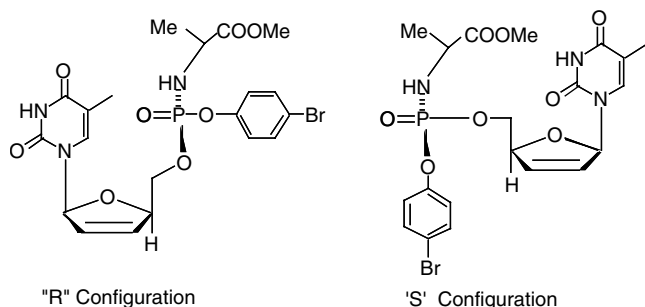
Figure 2. Structures of two individual isomers of stampidine.
